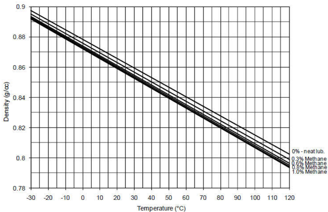
Figure 1. Density of BVAdvanced UPSI-5-68 / Methane
